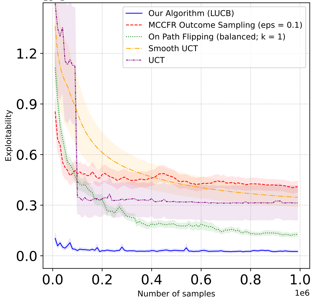
1e-1 Leduc Poker, Best Algorithms (new), Player x
